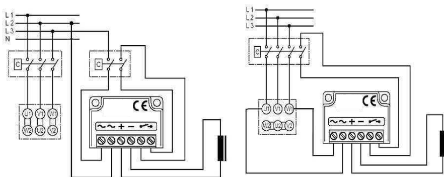
Connectin diagram from mains
