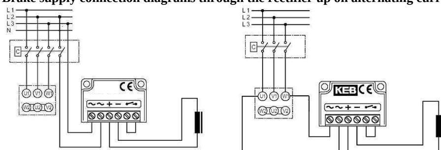
Connectin diagram from mains
