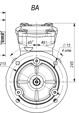
BAK100S2, S4 IM30x1
