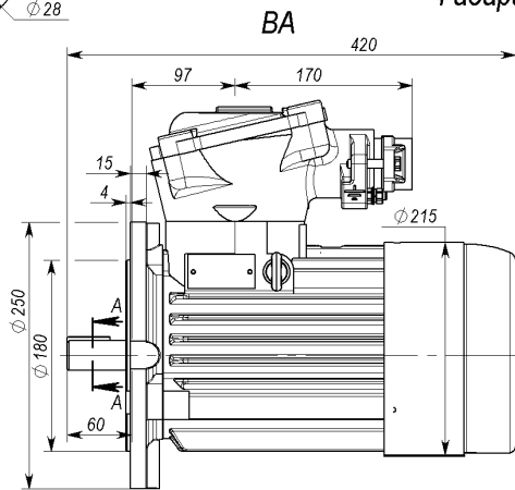
BAK100S2, S4 IM10x1
