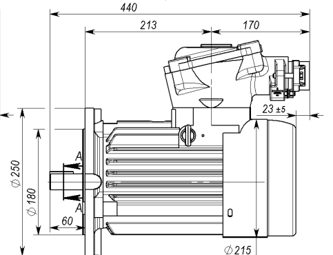
BAK100S2, S4 IM30x1
